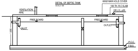
SECTION OF SEPTIC TANK SCALE: 1/50
