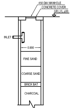
SECTION OF SOAK PIT SCALE: 1/50
